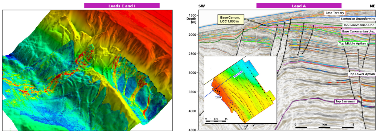
Illustration of Platform Edge Structural Prospects (Lead A)
